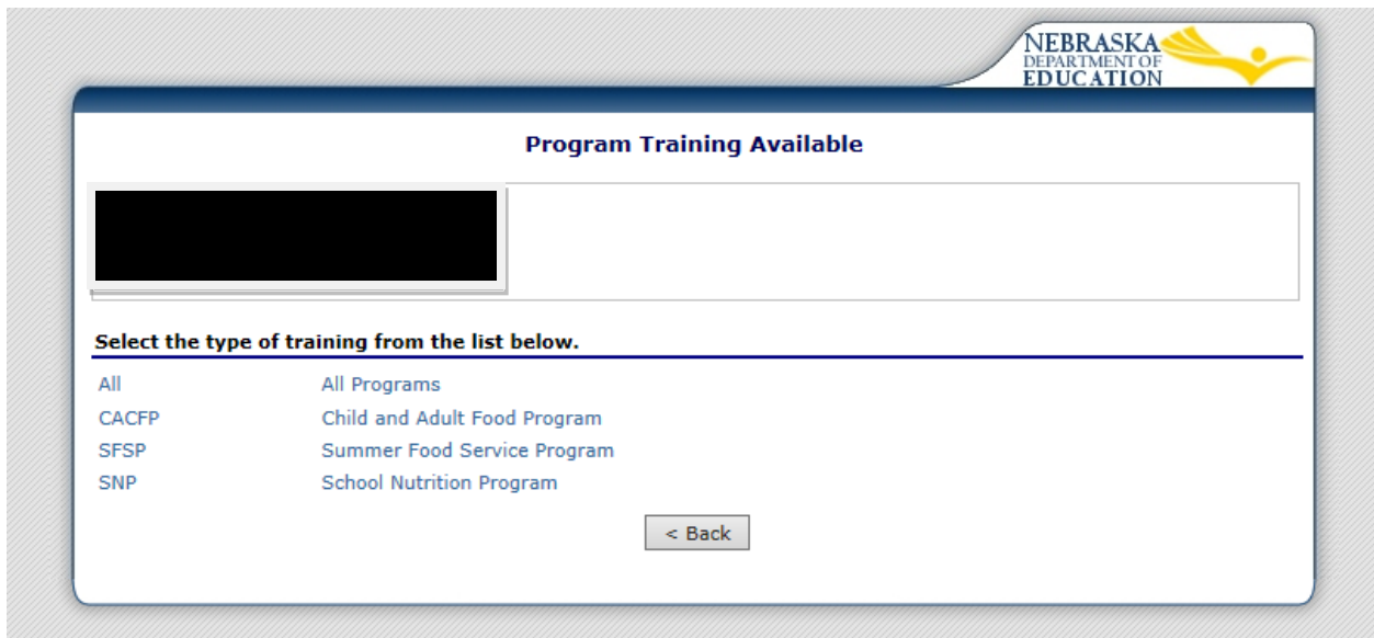
Figure 3. Program Trainings
